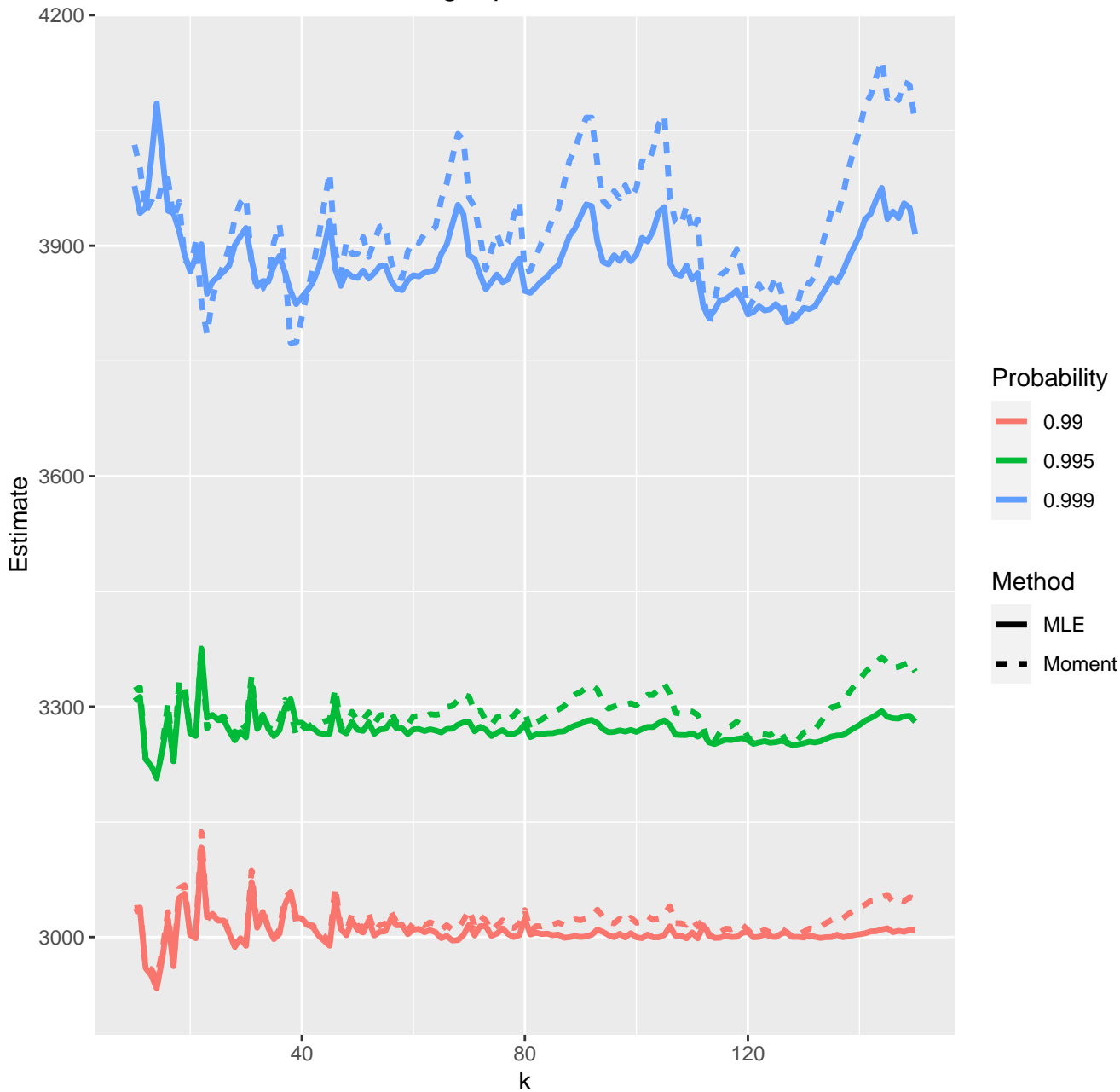
Estimates of high quantiles--13-01-2022
