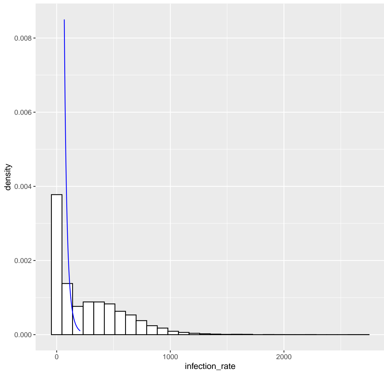
Fitted tail density GPD( 66.8 , 26.51 , 0.16 ), k= 80 -- 29-06-2021
