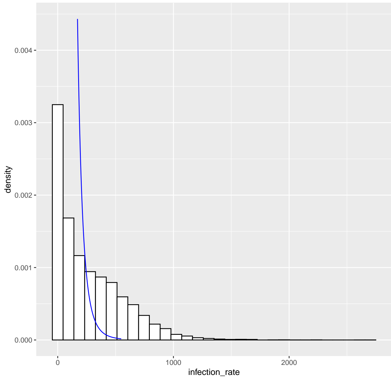
Fitted tail density GPD( 170.9 , 50.84 , 0.17 ), k= 80 -- 21-09-2021
