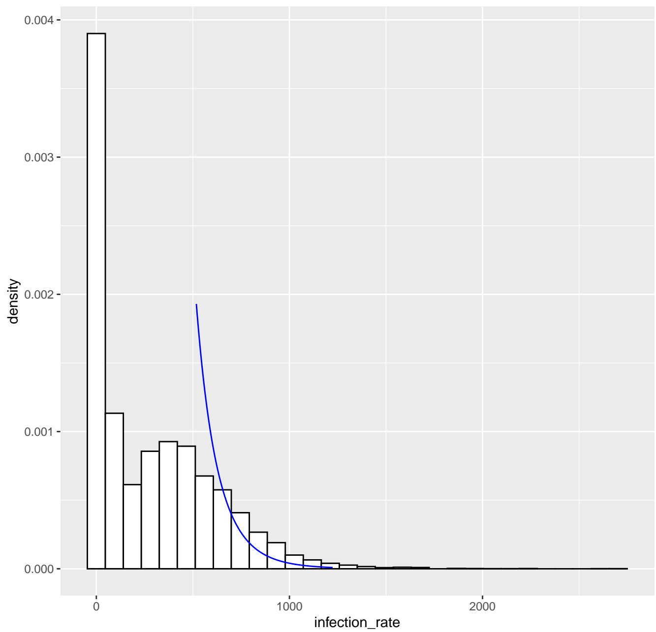
Fitted tail density GPD( 517.9 , 116.74 , 0.08 ), k= 80 -- 18-05-2021
