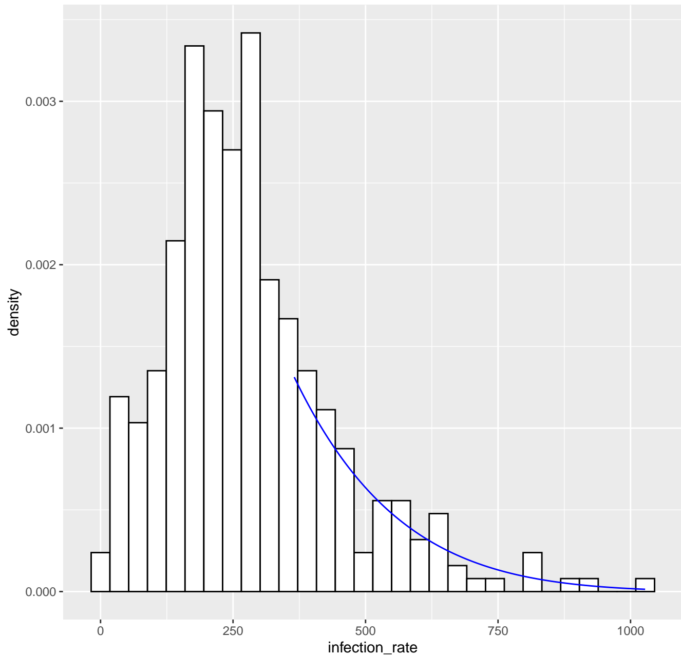
Fitted tail density GPD( 365.5 , 171.76 , -0.12 ), k= 80 -- 14-06-2020
