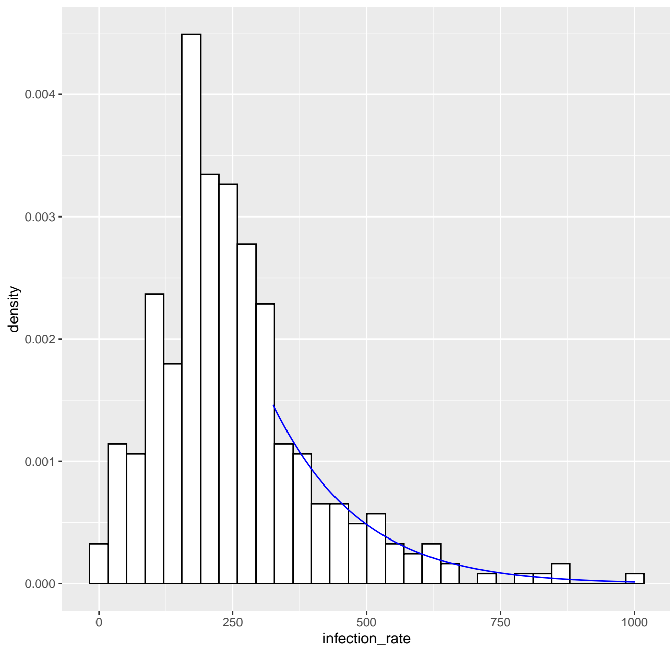
Fitted tail density GPD( 325.4 , 154.14 , -0.05 ), k= 80 -- 10-05-2020
