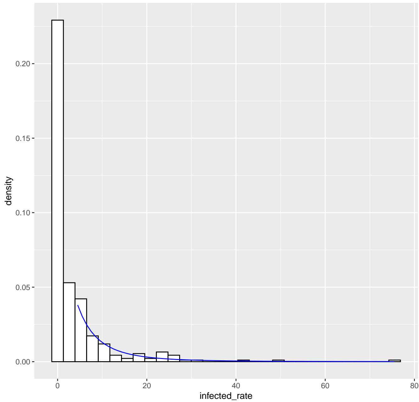
Fitted tail density GPD( 4.51 , 5.93 , 0.34 ), k= 80 -- 12-03-2020
