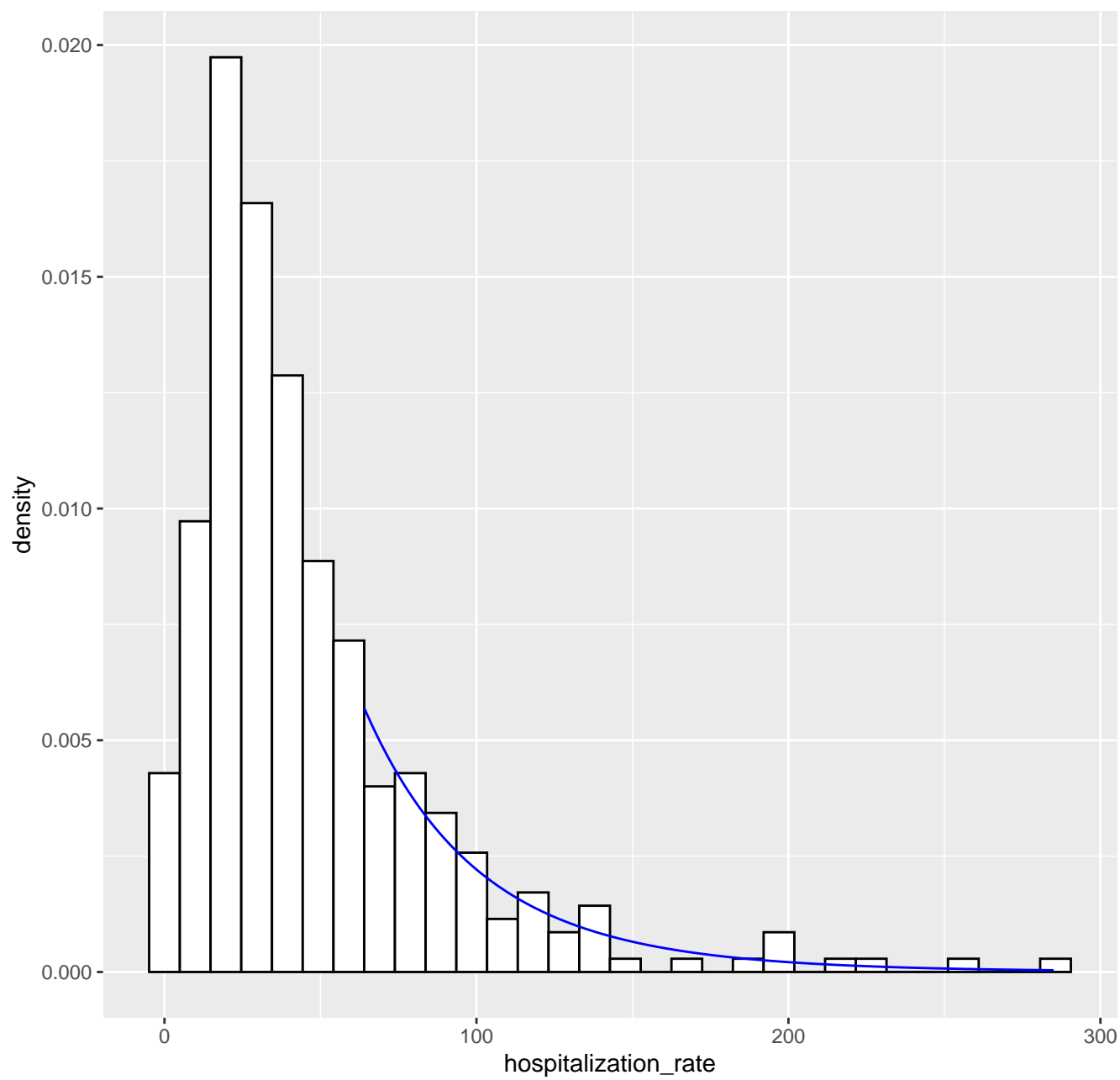
Fitted tail density GPD( 64 , 39.53 , 0.08 ), k= 80 -- 07-04-2020
