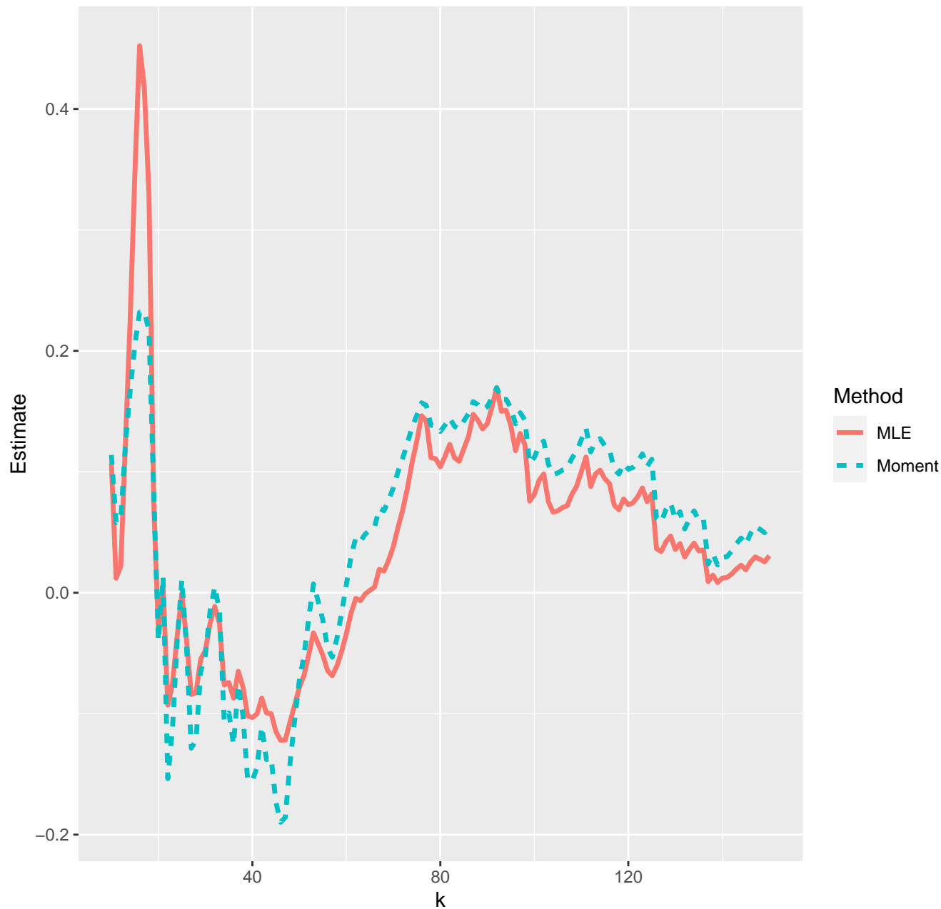
Estimates of extreme value index--29-12-2020
